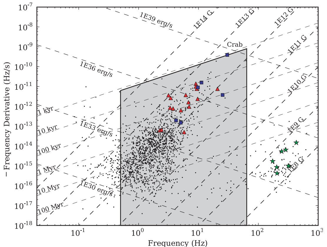
Fig. 1. Frequency ( f ) and frequency derivative ( \dot{f} ) distribution of the new pulsars. The dots represent the \sim 1800 pulsars in the ATNF catalog (20), the triangles represent the new pulsars reported here, and the squares represent the six previously known EGRET gamma-ray pulsars, including the Crab. The stars represent the new population of gamma-ray millisecond pulsars detected by the Fermi LAT and reported in (10). The shaded region shows the parameter space covered by our blind search and includes \sim 86\% of the ATNF pulsars. The three sets of lines illustrate the characteristic age \tau = -f/2\dot{f} , inferred surface magnetic field strength B = 3.2 \times 10^{19} \sqrt{-\dot{f}/f^3} G, and spin-down power given by \dot{E} = 4\pi^2 I f \dot{f} ergs s ^{-1} , where I is the neutron star moment of inertia ( I = 10^{45} g cm ^2 ). This figure shows that the blind-search gamma-ray pulsars are drawn from the portion of the general population with the highest spin-down luminosity.
